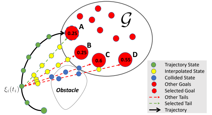
Fig. 3: Online goal selection algorithm at the i th iteration. The goal costs c(g) are denoted inside red circles. In this example, the online learning algorithm is about to shift goal from A to B , which yields a collision-free yet shorter trajectory.
