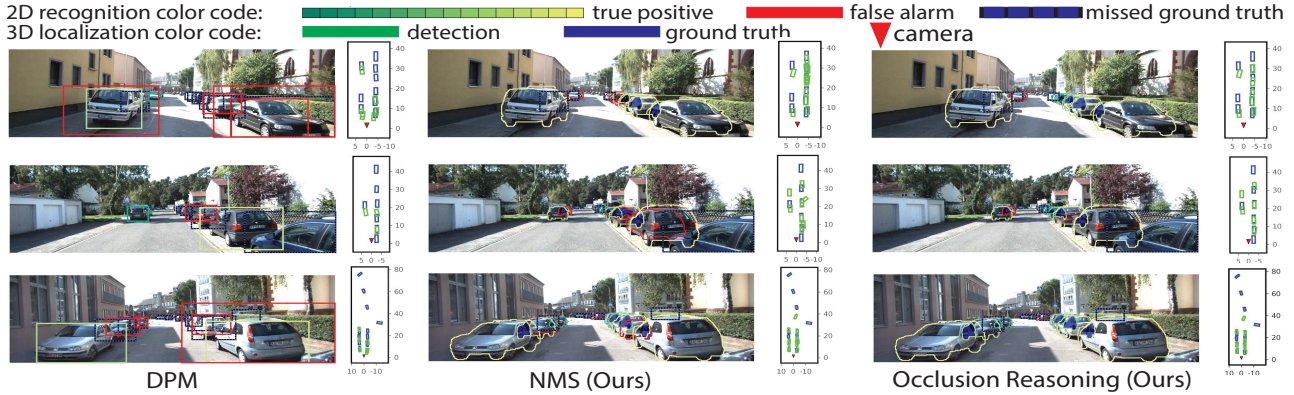
Figure 7. Car recognition results on the KITTI validation set. We compare our method w/o occlusion reasoning and DPM [10]. Detections at 1 false positive per image (fppi) for the three methods are shown. Blue regions in the images are the estimated occluded areas. Note that severe false alarms in NMS disappear with occlusion reasoning.
